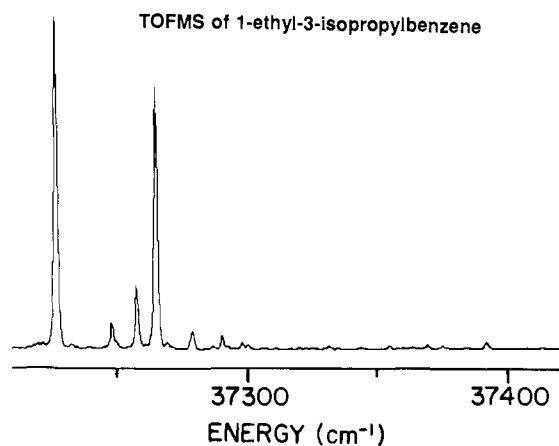
Figure 10. TOFMS of the 0_0^0 region of the S_1 \leftarrow S_0 transition of 1-ethyl-3-isopropylbenzene (21). The two origins of the spectrum, at 37226.6 and 37264.8 \text{ cm}^{-1} , help identify the stable conformation of the isopropyl group as 17, as outlined in the text.
