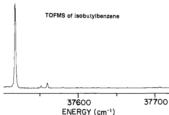
Figure 3. TOFMS of the 0 0 0 region of the S 1 ← S 0 transition of isobutylbenzene ( 7 ). The spectrum displays a single origin at 37517.8 cm -1 . The weak features at 37551.4 and 37559.6 cm -1 are attributed to torsional motion of the isobutyl group.
