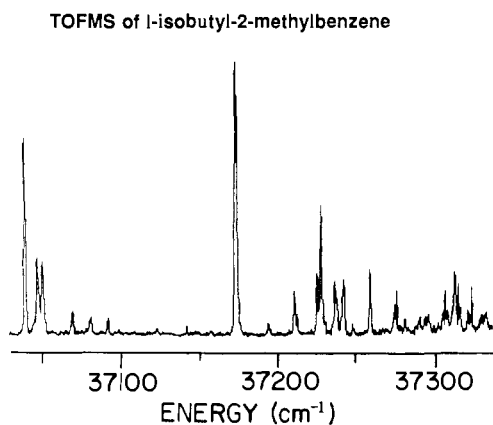
Figure 5. TOFMS of the 0_0^0 region of 1-isobutyl-2-methylbenzene ( 11 ). Two origins are observed in the spectrum at 37036.0 and 37171.8 cm -1 .
