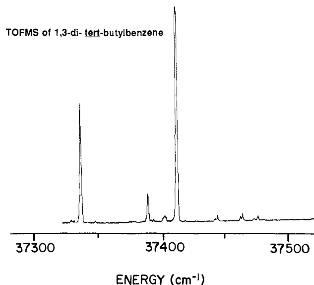
Figure 17. TOFMS of 1,3-di- tert -butylbenzene ( 45 ). The three most intense peaks in the spectrum at 37 335.6, 37 388.1, and 37 410.2 cm -1 are assigned to three different spectroscopy origins corresponding to three stable conformations for this molecule.
