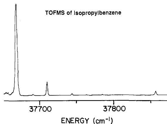
Figure 8. TOFMS of the 0_0^0 region for the S_1 \leftarrow S_0 transition of isopropylbenzene ( 16 ). The sole origin occurs at 37668.5 \text{ cm}^{-1} . The weaker feature at 37710.0 \text{ cm}^{-1} is attributed to torsional motion of the isopropyl group.
