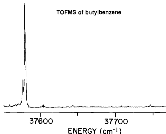
Figure 7. TOFMS of the 0_0^0 region of the S_1 \leftarrow S_0 transition of butylbenzene ( 13 ). The intense feature at 37581.8 cm -1 is assigned to the staggered, all-anti conformation of the butyl group ( 14aa ). The weaker feature at 37578.0 cm -1 is also assigned as a separate origin, corresponding to 14ag .
