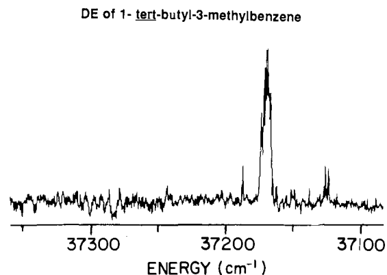
Figure 16. DE spectrum for 1- tert -butyl-3-methylbenzene ( 42 ) obtained by pumping the 37 169.8-cm -1 feature in Figure 15a. Resolution is 7.6 cm -1 . The absence of a feature to higher energy of the peak at 37 169.8 cm -1 helps to preclude the assignment of the 37 169.8-cm -1 feature in Figure 15, a and b, as a hot band.
