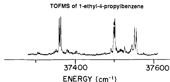
Figure 2. TOFMS of the 0_0^0 region of 1-ethyl-4-propylbenzene (4). The spectrum consists of four origins at 37369.1, 37372.7 and 37496.7, 37497.3 \text{cm}^{-1} , corresponding to four stable conformations for this molecule (see text).
