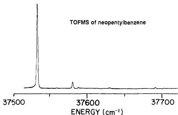
Figure 6. TOFMS of the 0_0^0 region of neopentylbenzene ( 12 ). The spectrum shows only one origin at 37533.6 cm -1 . Weaker features, higher in energy than the origin, are attributed to low-frequency torsional motions of the neopentyl group.
