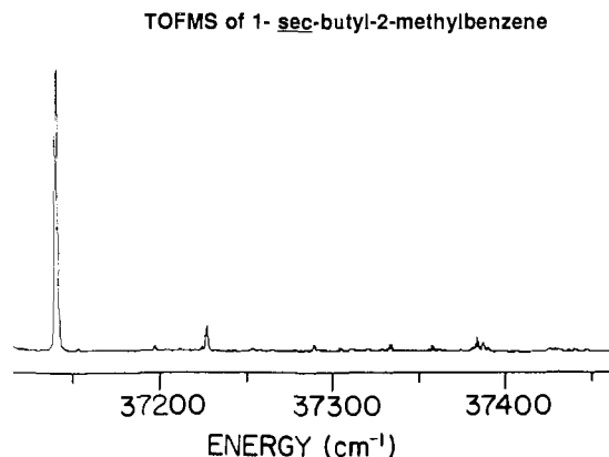
Figure 12. TOFMS of the 0_0^0 region of 1- sec -butyl-2-methylbenzene ( 30 ). The spectrum contains only a single origin. This is consistent with MOMM calculation which predicts only one stable conformation for this molecule (see text).
