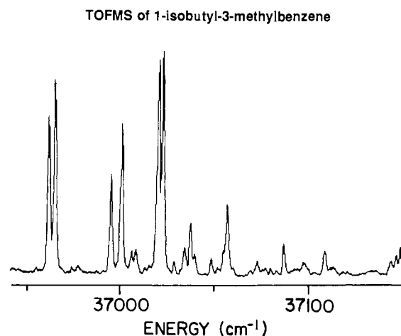
Figure 4. TOFMS of the 0 0 0 region of the S 1 ← S 0 transition of 1-isobutyl-3-methylbenzene ( 10 ). The spectrum contains two origins at 36965.1 and 37023.0 cm -1 . The peaks occurring 3 cm -1 lower in energy than these origins are due to ring methyl torsions.
